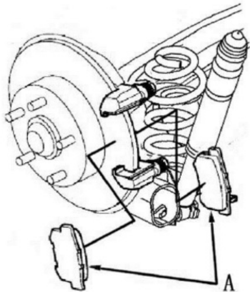
(4) 拆下卡钳簧片 (A)
