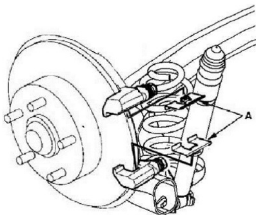
(4) 拆下卡钳簧片 (A)
